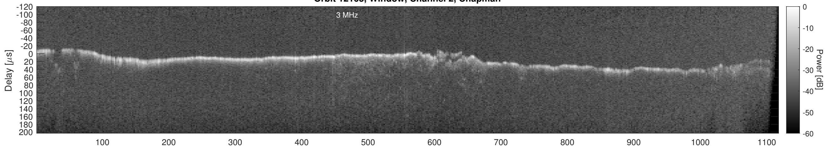
Orbit 12163, Window, Channel 2, Optimized
