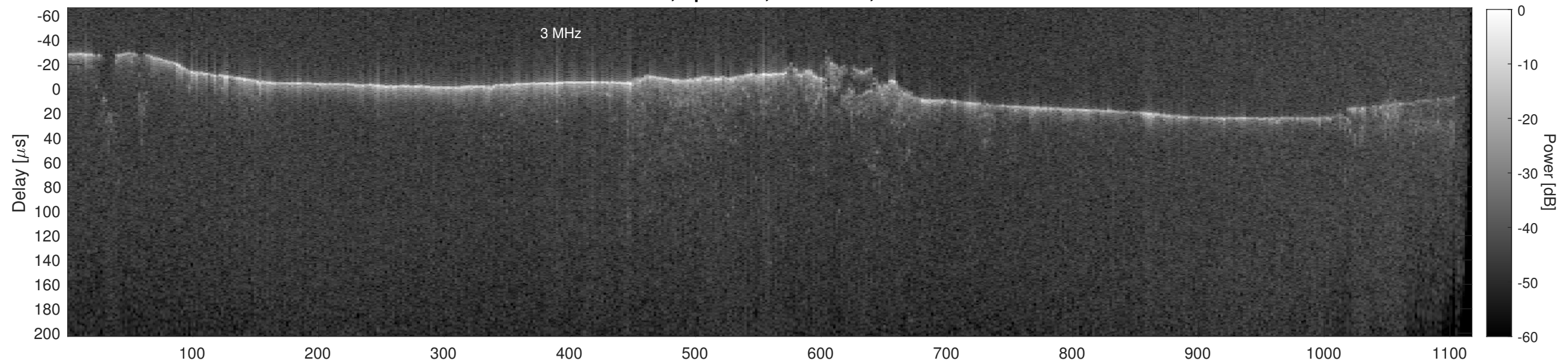
Orbit 12163, Cluttergram
