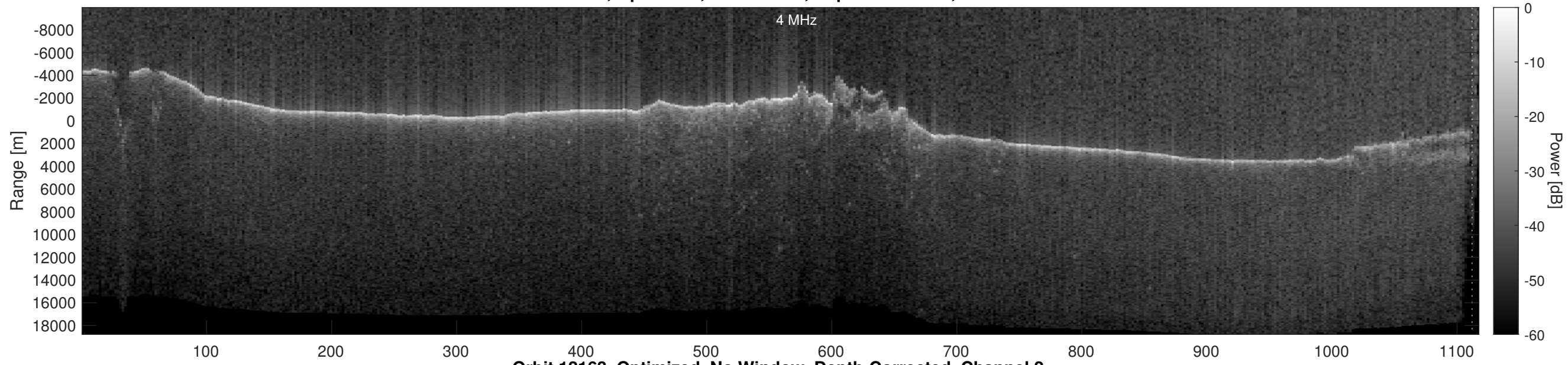
Orbit 12163, Optimized, No Window, Depth-Corrected, Channel 2
