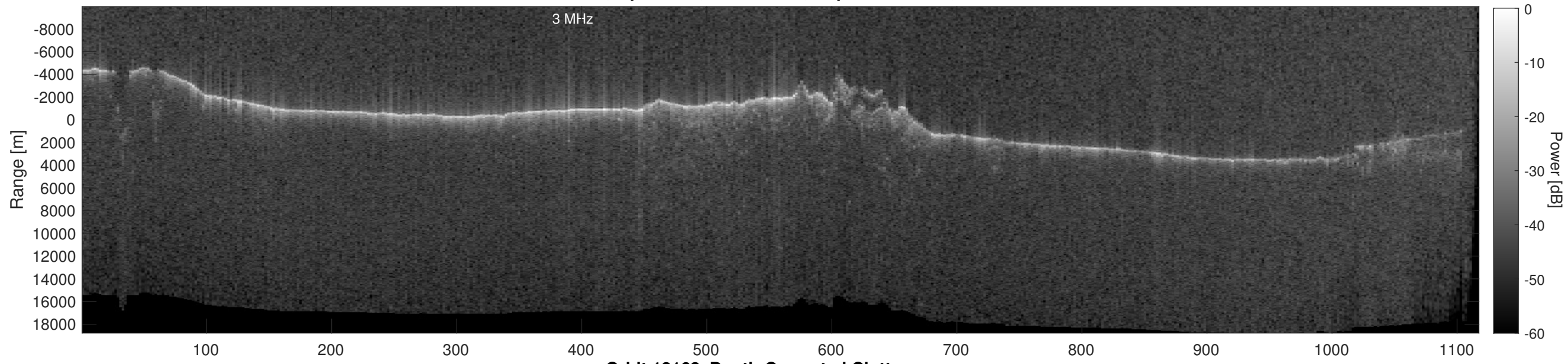
Orbit 12163, Depth-Corrected Cluttergram
