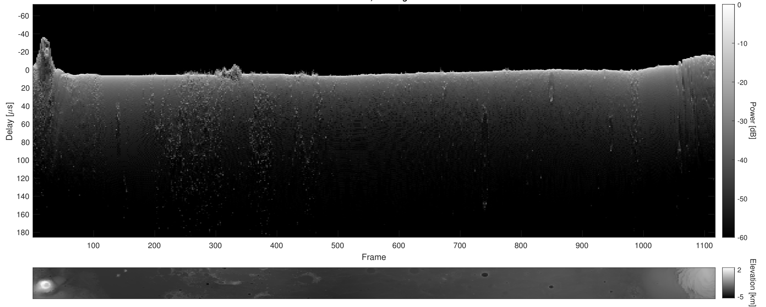
Orbit 12164, Cluttergram
