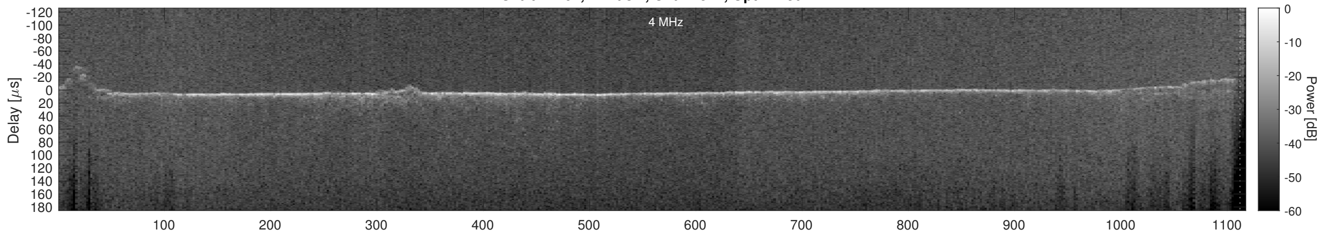
Orbit 12164, Cluttergram
