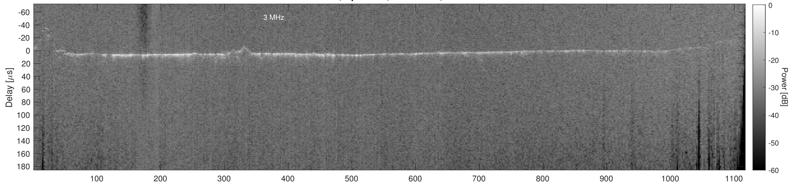
Orbit 12164, Cluttergram
