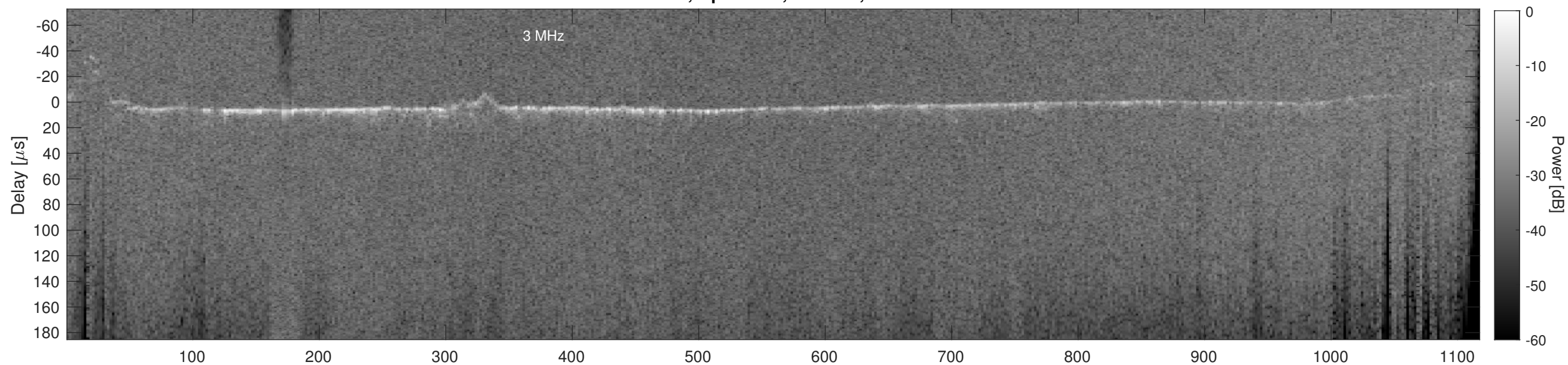
Orbit 12164, Cluttergram
