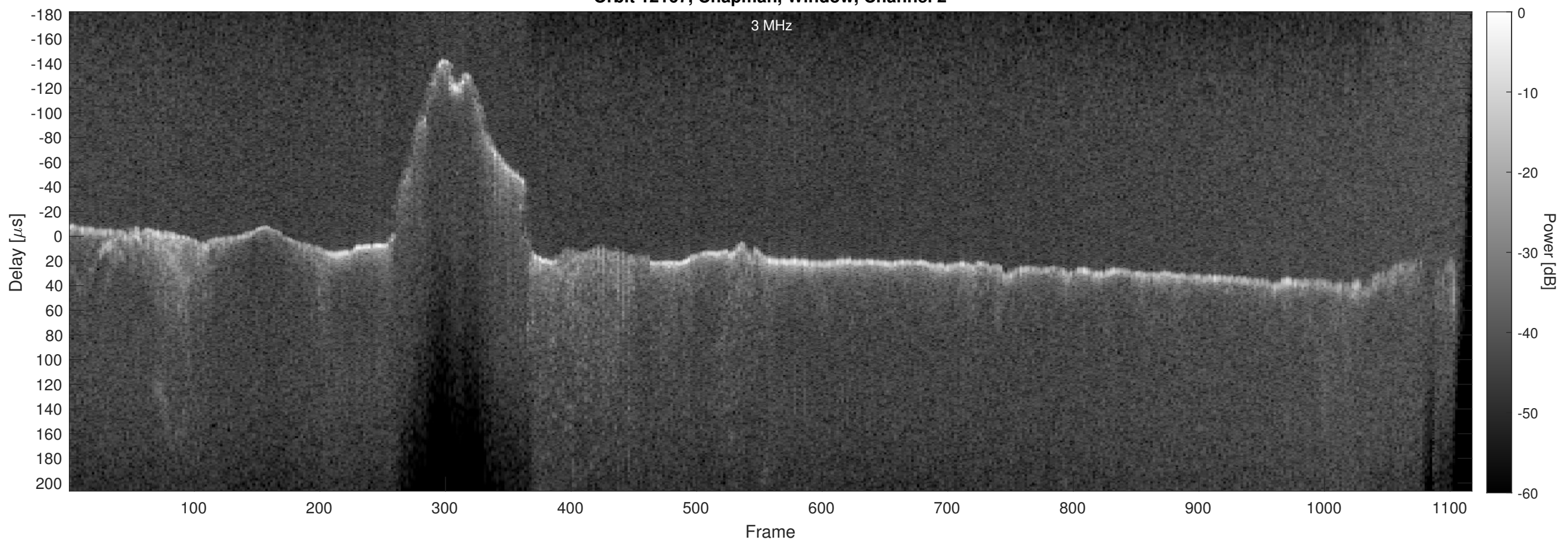
Orbit 12167, Chapman, Window, Channel 2
