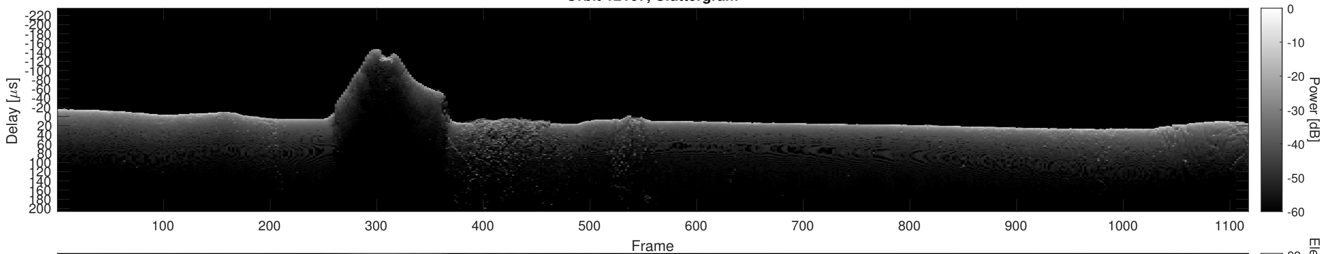
Orbit 12167, Cluttergram
