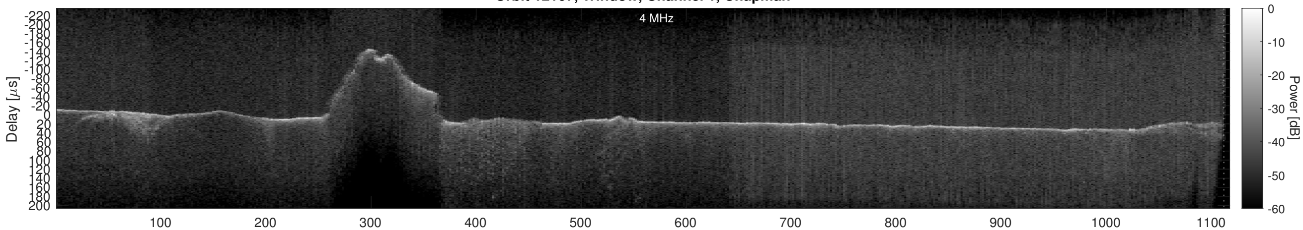
Orbit 12167, Window, Channel 1, Optimized
