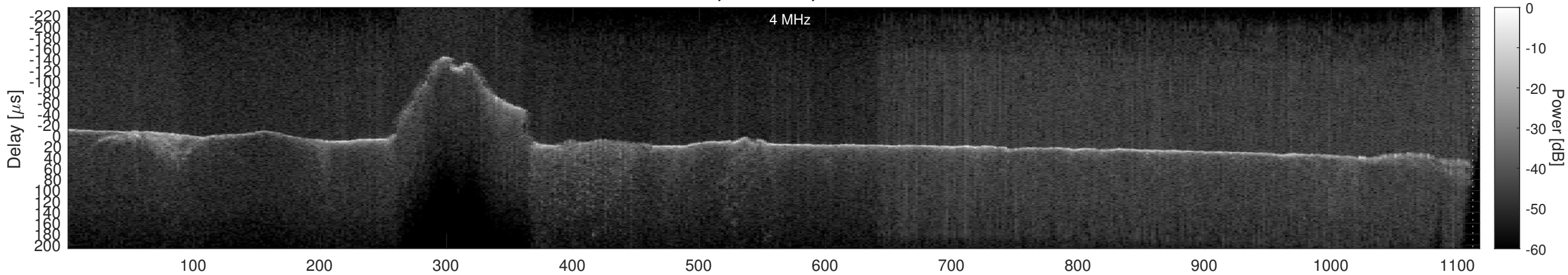
Orbit 12167, Window, Channel 1, Chapman
