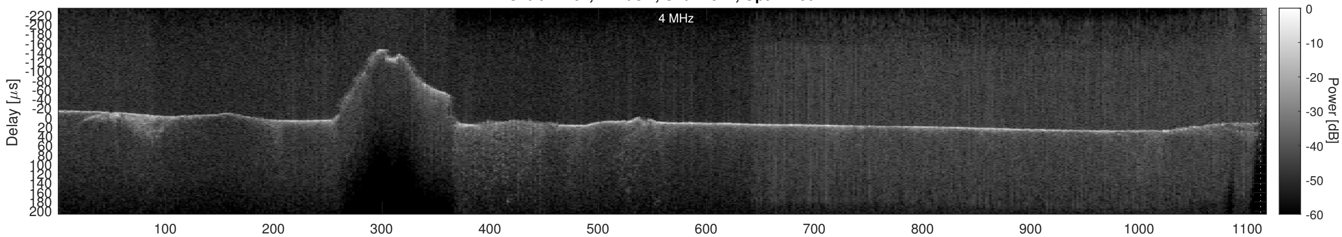
Orbit 12167, Cluttergram
