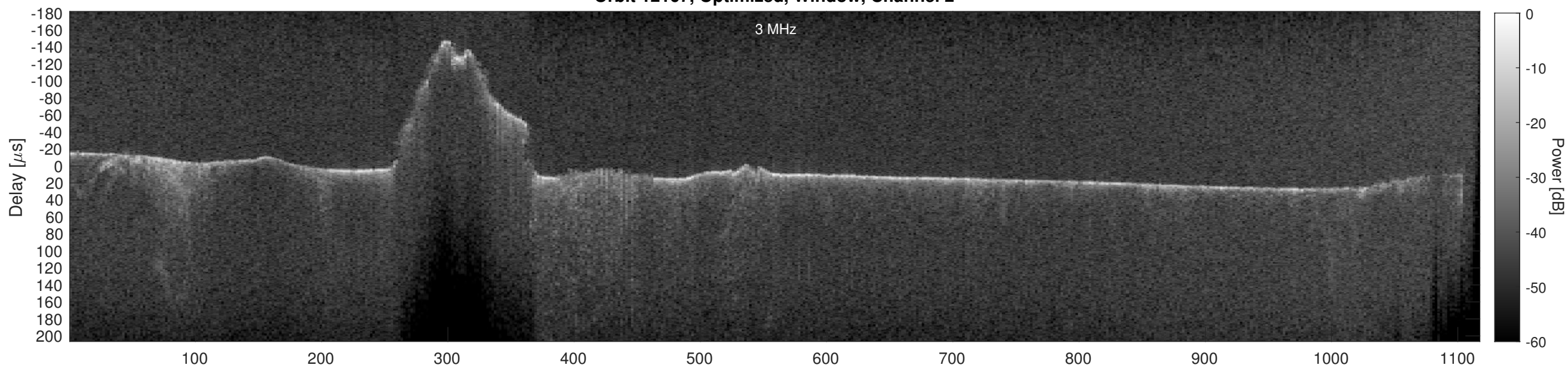
Orbit 12167, Cluttergram
