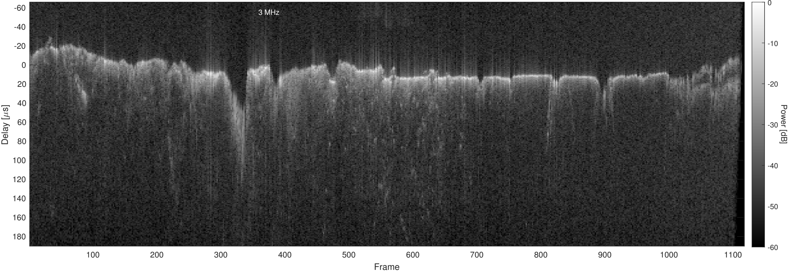
Orbit 12169, Chapman, No Window, Channel 2
