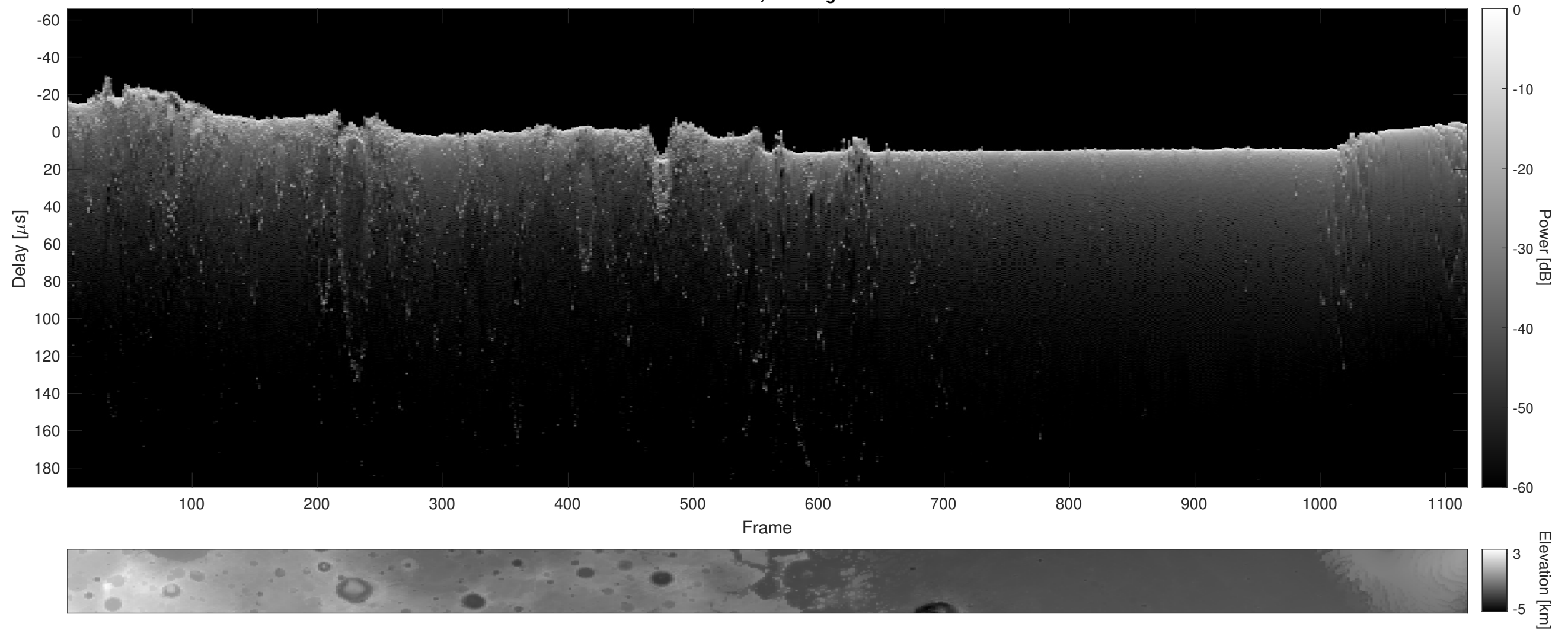
Orbit 12169, Cluttergram
