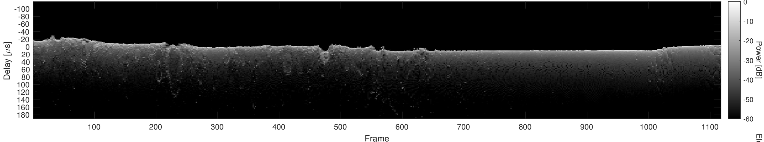
Orbit 12169, Cluttergram
