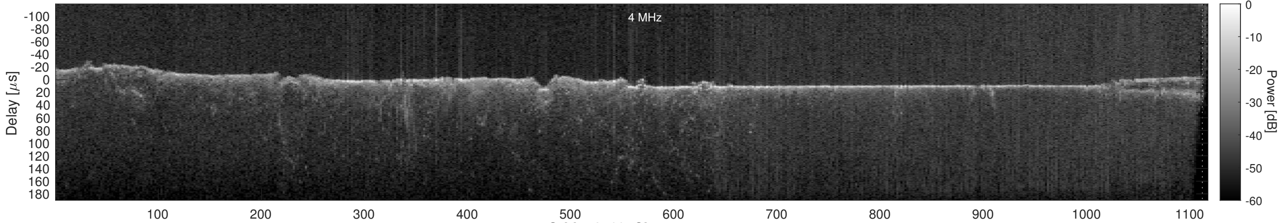
Orbit 12169, Cluttergram
