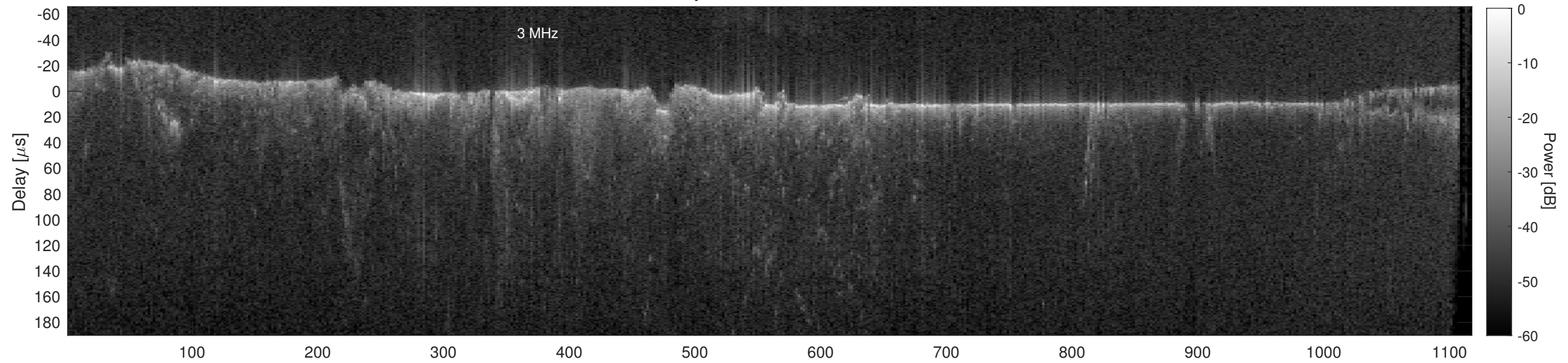
Orbit 12169, Cluttergram
