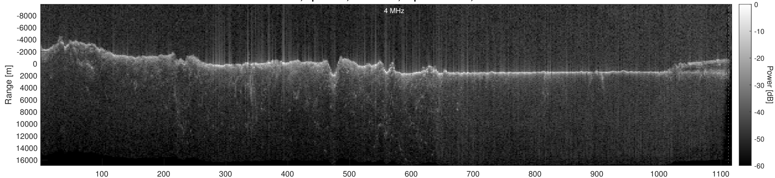
Orbit 12169, Optimized, No Window, Depth-Corrected, Channel 2
