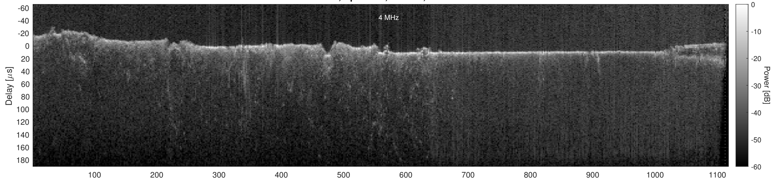
Orbit 12169, Optimized, Window, Channel 2
