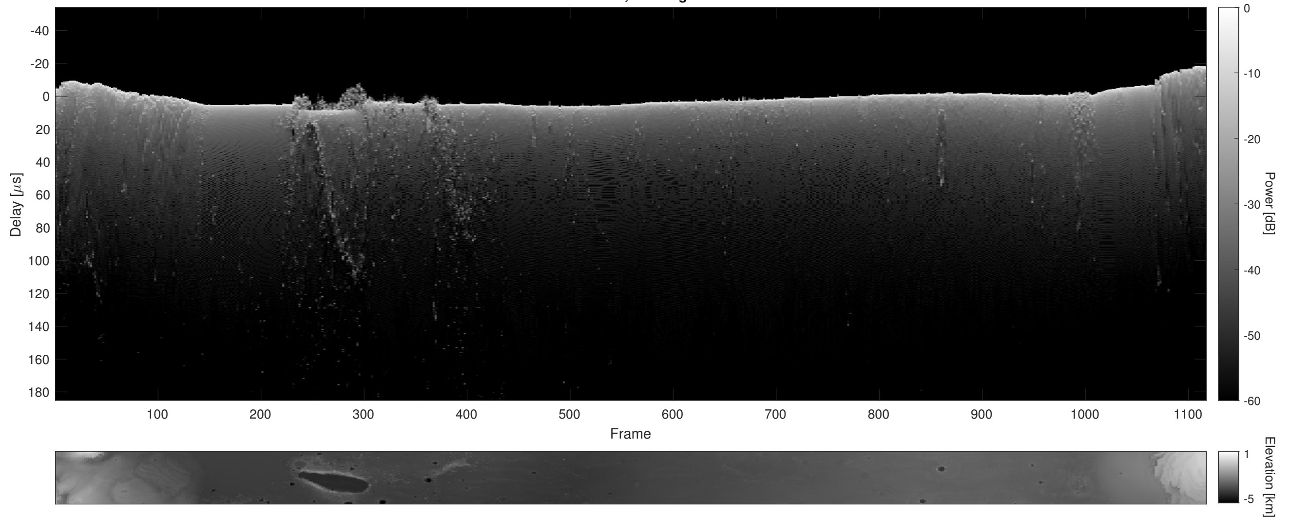
Orbit 12171, Cluttergram
