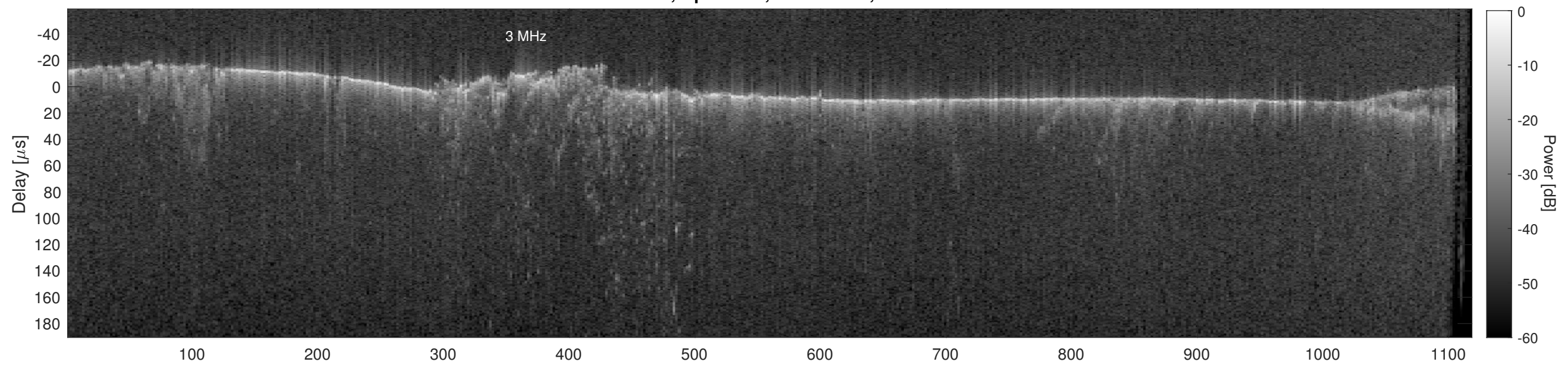
Orbit 12172, Cluttergram
