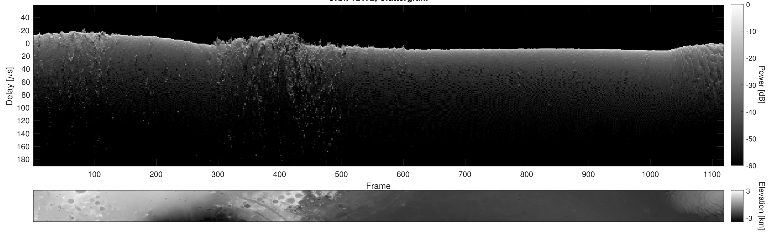
Orbit 12172, Cluttergram
