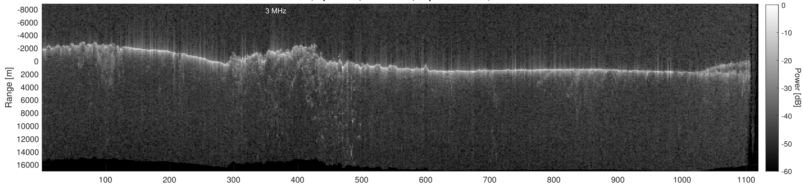
Orbit 12172, Depth-Corrected Cluttergram
