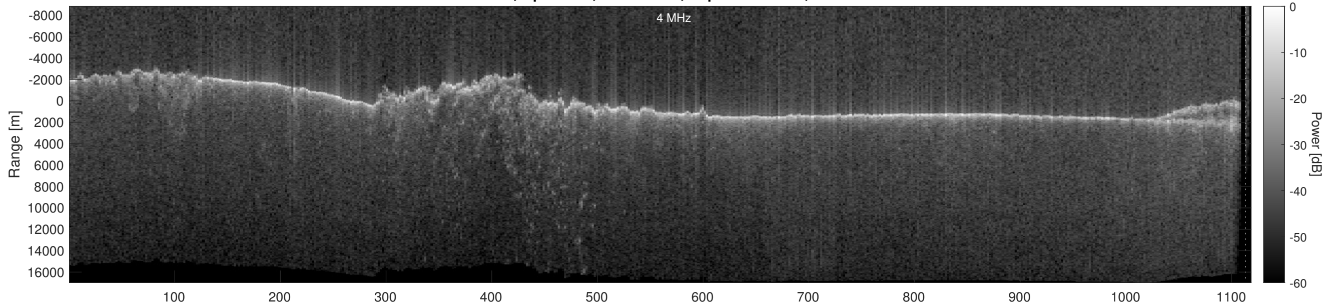
Orbit 12172, Optimized, No Window, Depth-Corrected, Channel 2
