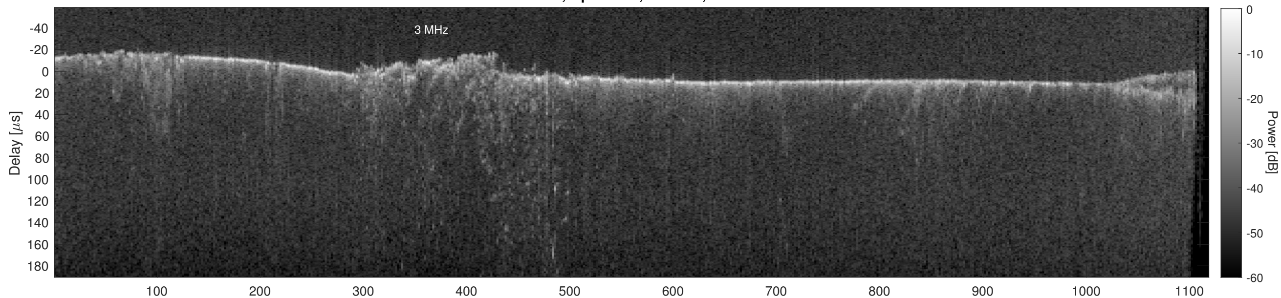
Orbit 12172, Cluttergram
