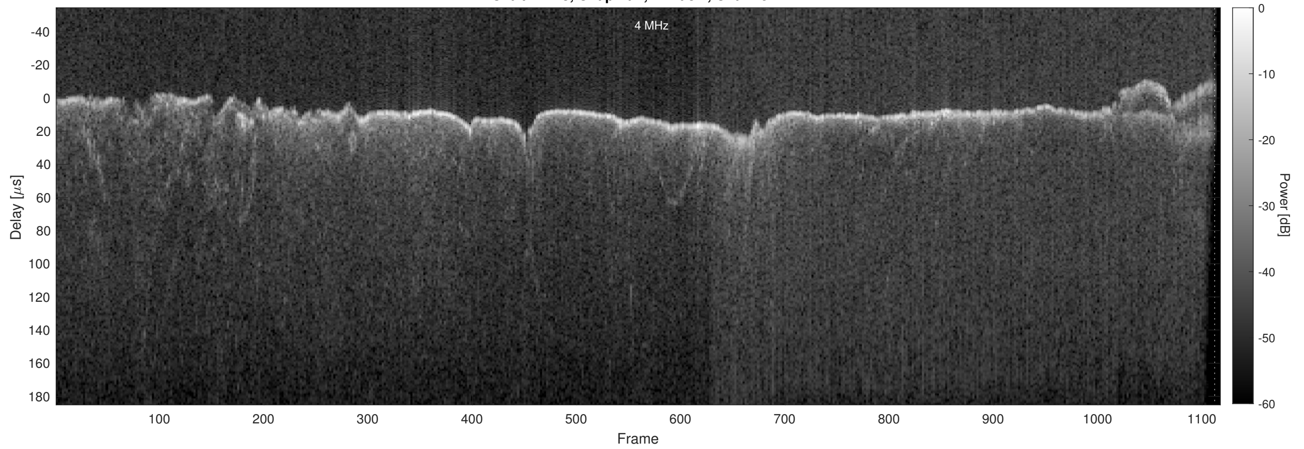
Orbit 12173, Chapman, Window, Channel 2
