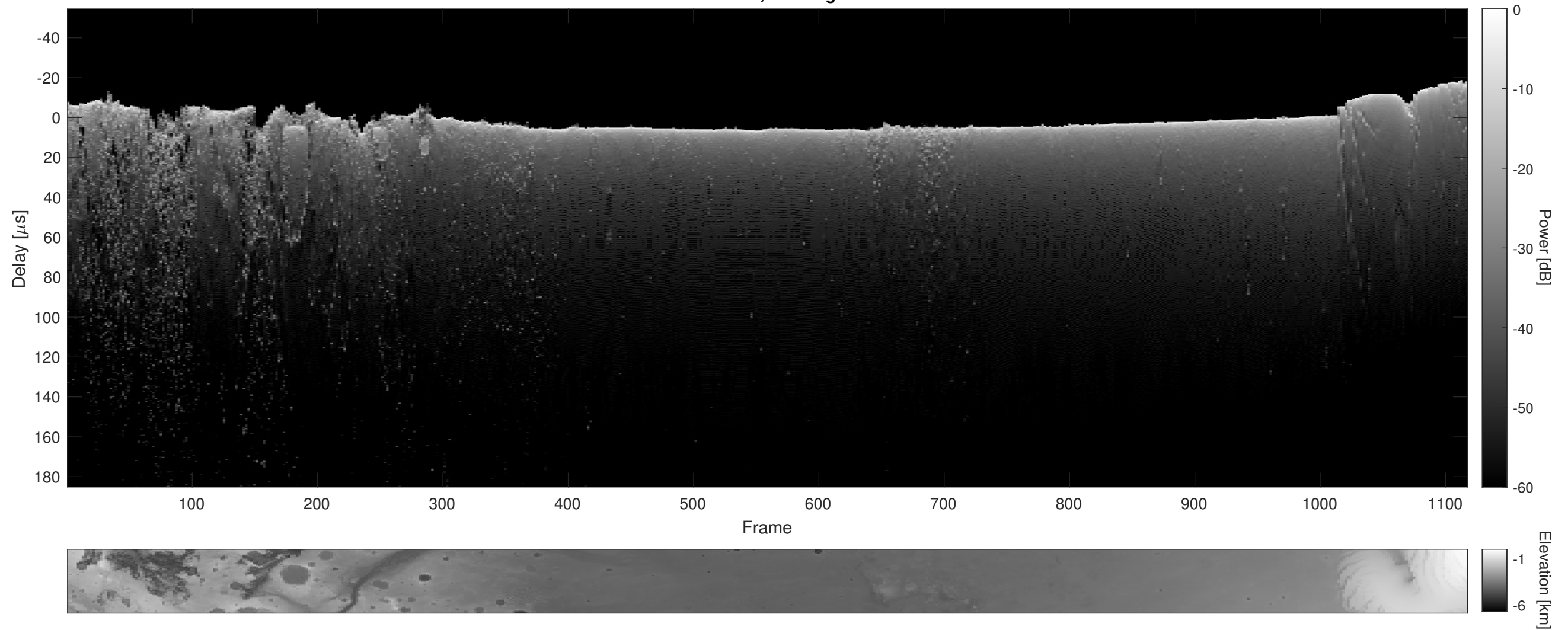
Orbit 12173, Cluttergram
