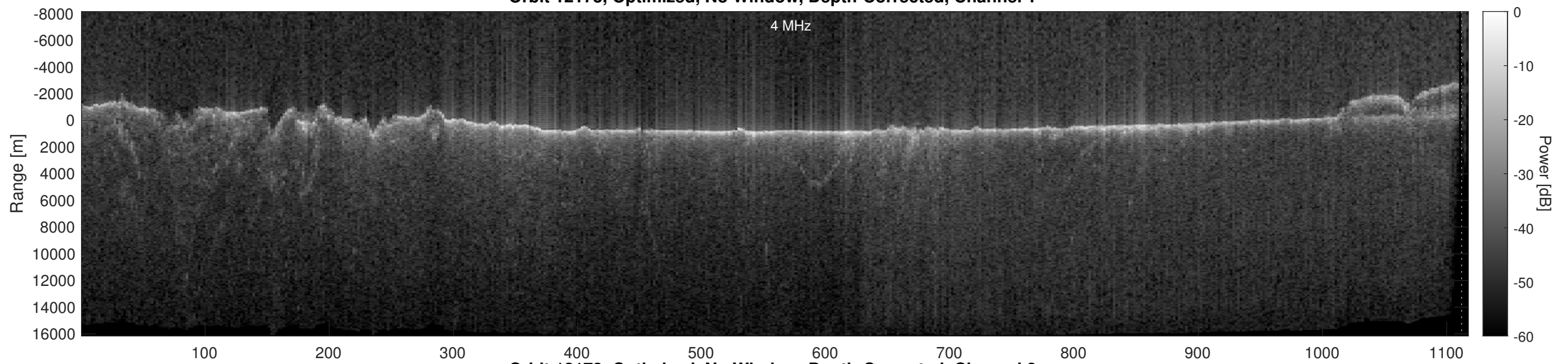
Orbit 12173, Optimized, No Window, Depth-Corrected, Channel 2
