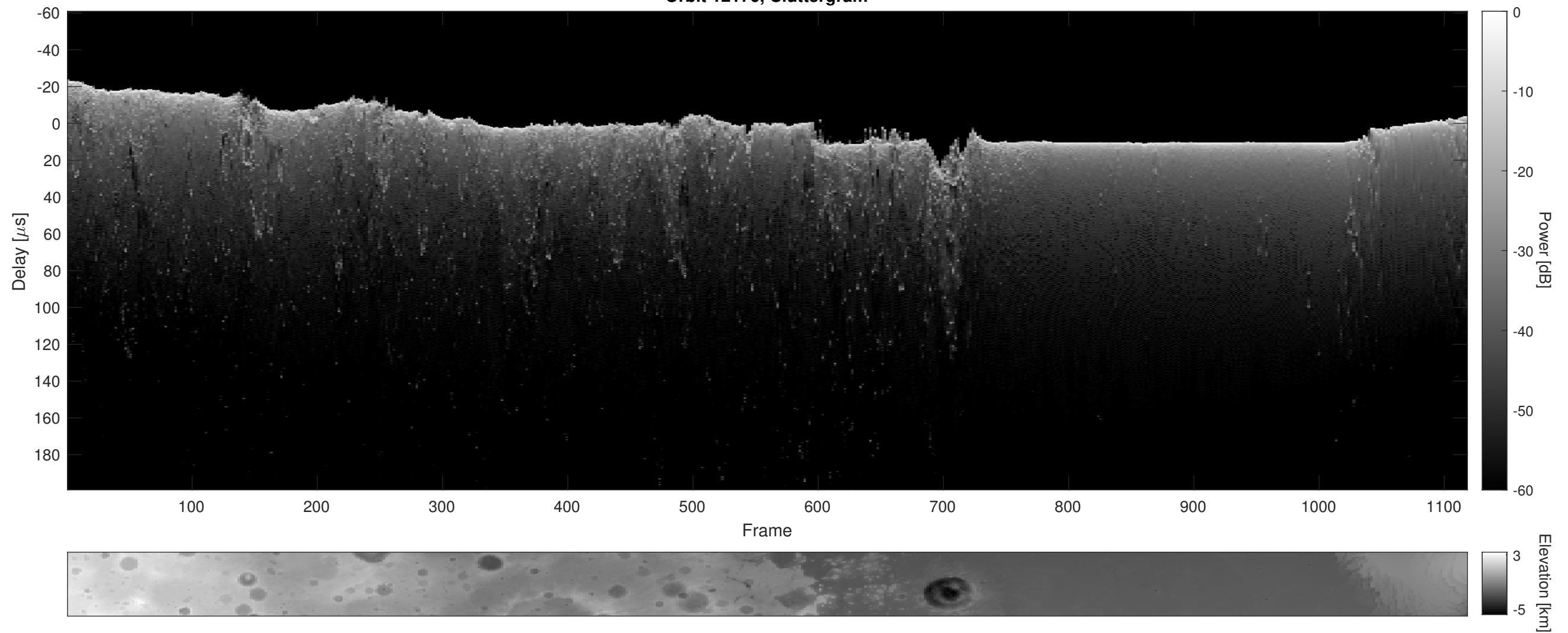
Orbit 12176, Cluttergram
