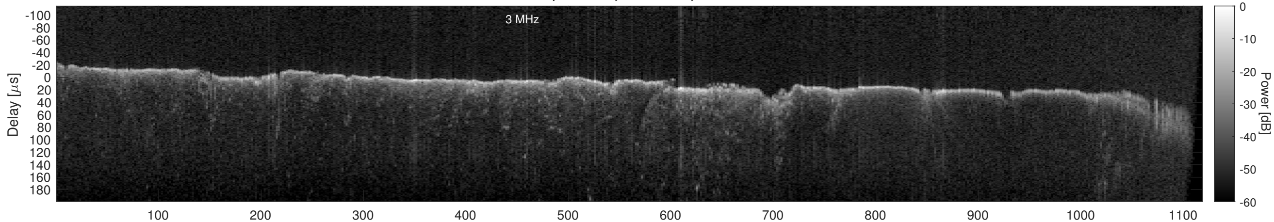
Orbit 12176, Window, Channel 2, Chapman
