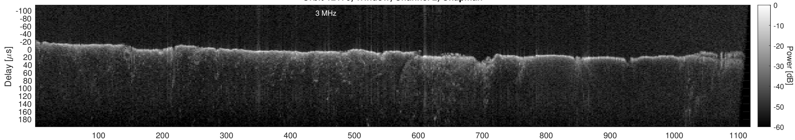
Orbit 12176, Window, Channel 2, Optimized
