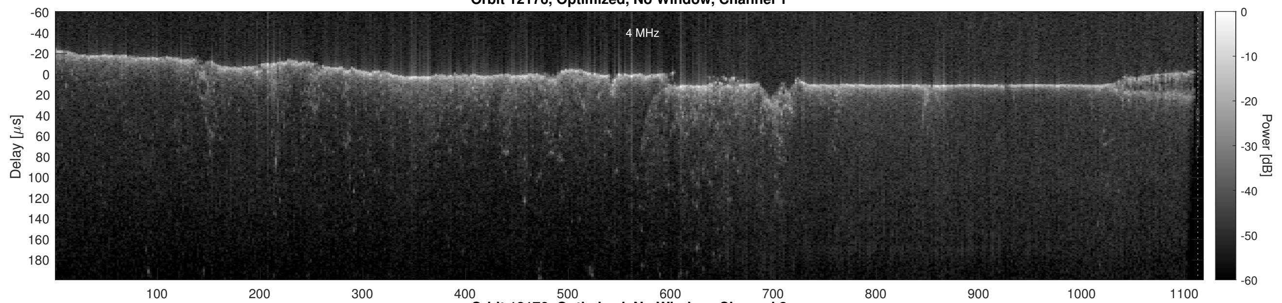
Orbit 12176, Optimized, No Window, Channel 2
