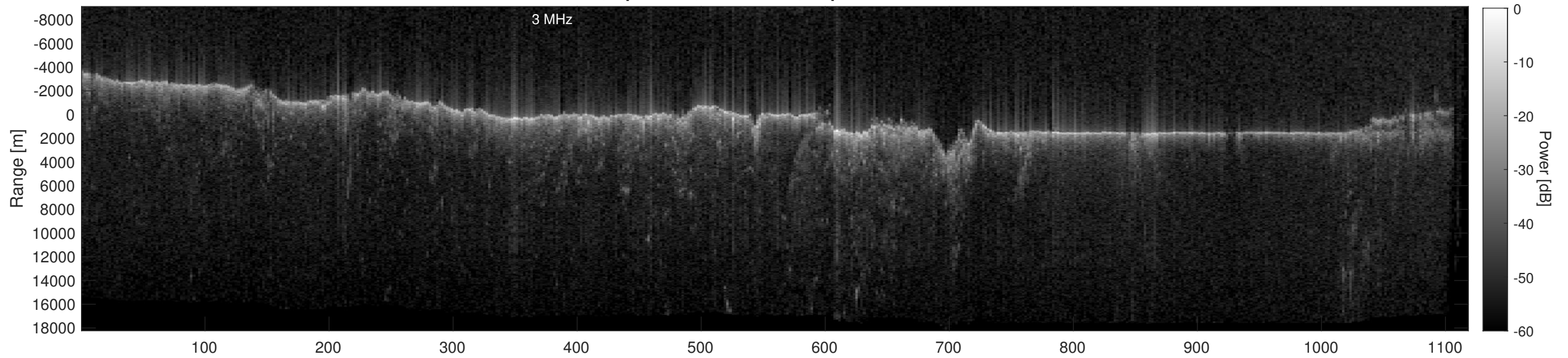
Orbit 12176, Depth-Corrected Cluttergram
