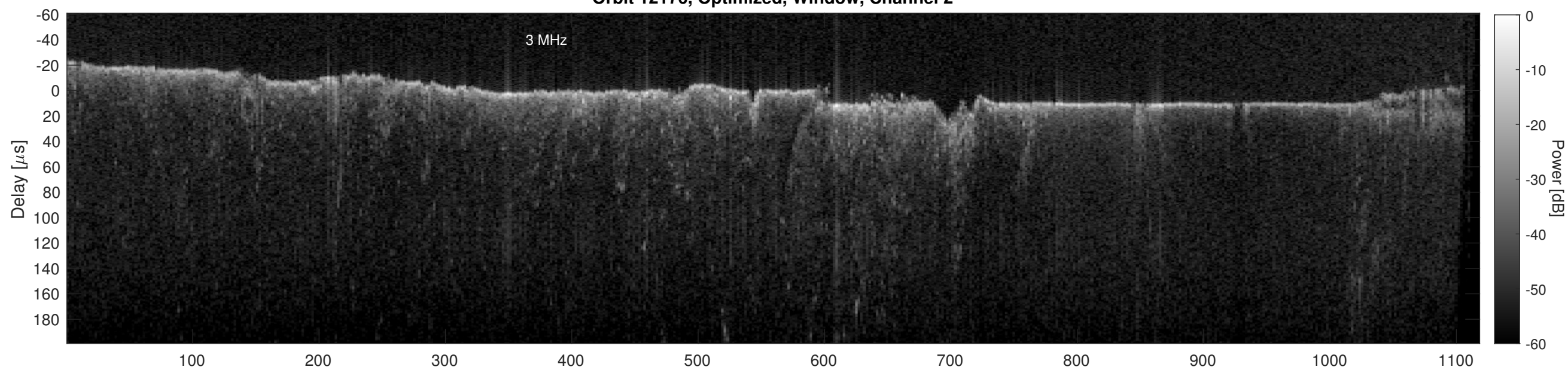
Orbit 12176, Cluttergram
