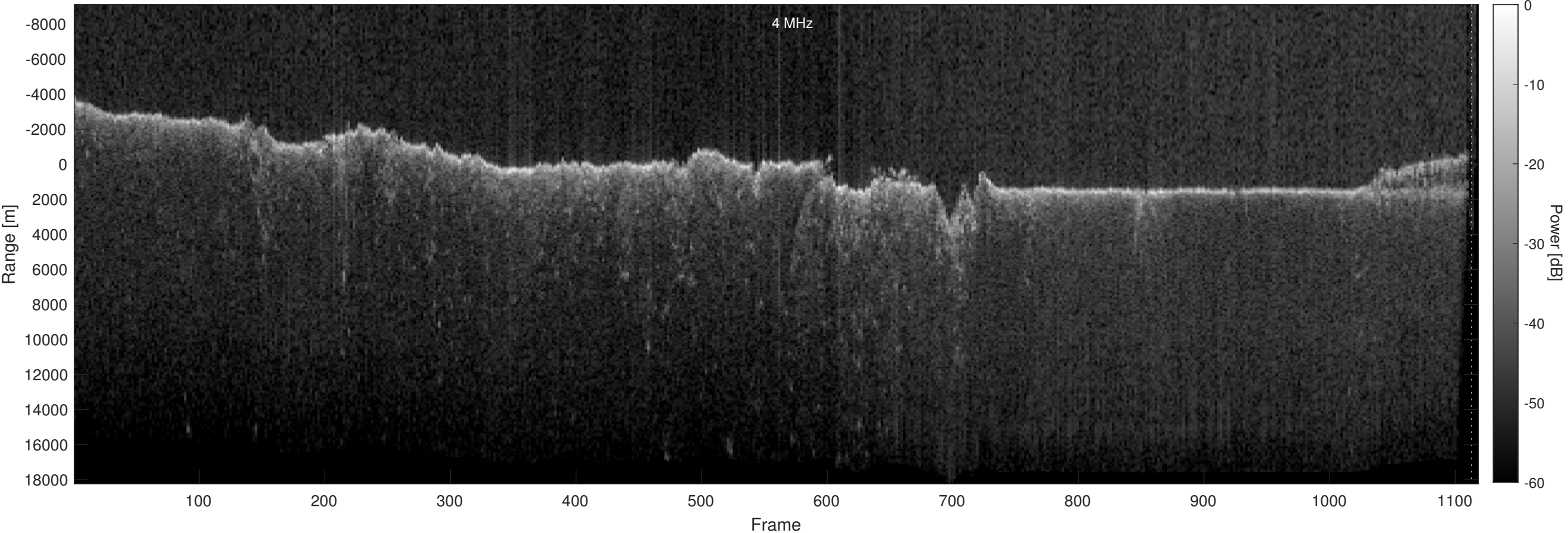
Orbit 12176, Optimized, Window, Depth-Corrected, Channel 2
