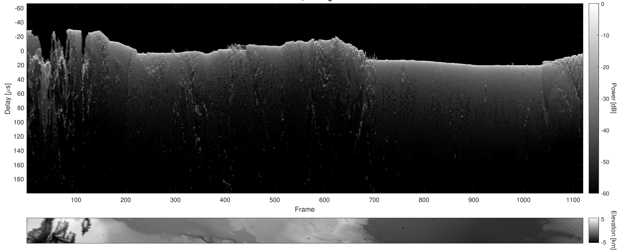
Orbit 12177, Cluttergram
