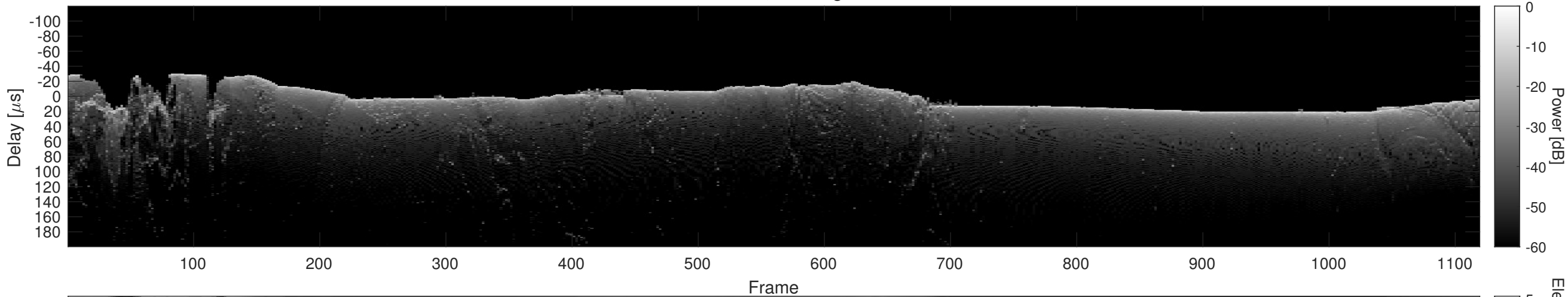
Orbit 12177, Cluttergram
