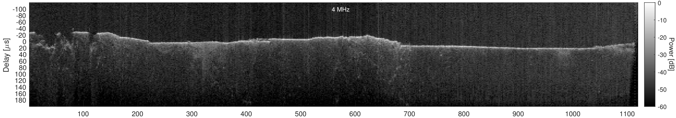
Orbit 12177, Cluttergram
