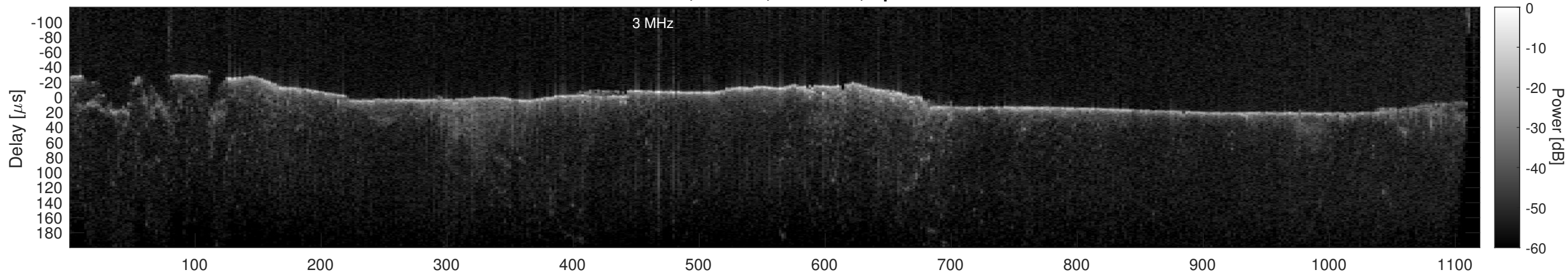
Orbit 12177, Cluttergram
