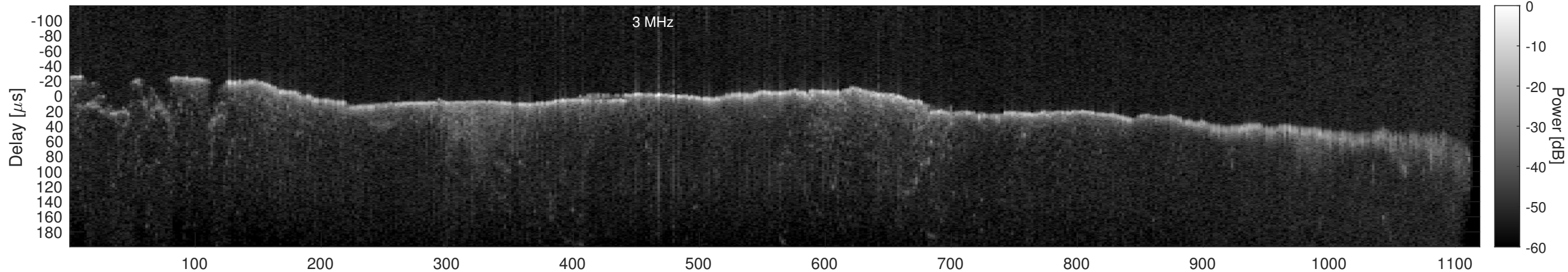
Orbit 12177, Window, Channel 2, Chapman
