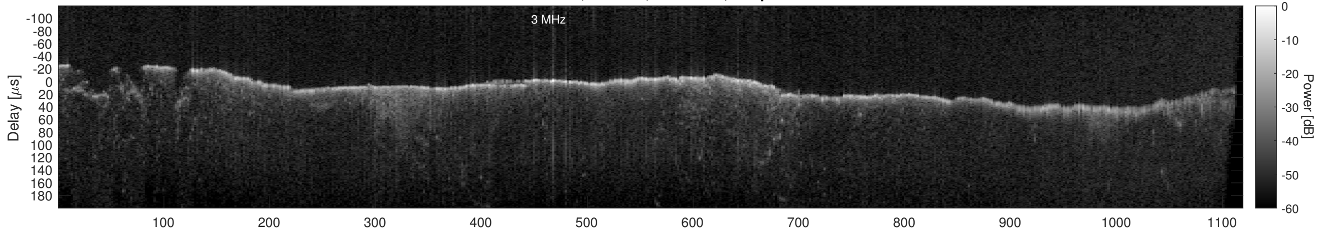
Orbit 12177, Window, Channel 2, Optimized
