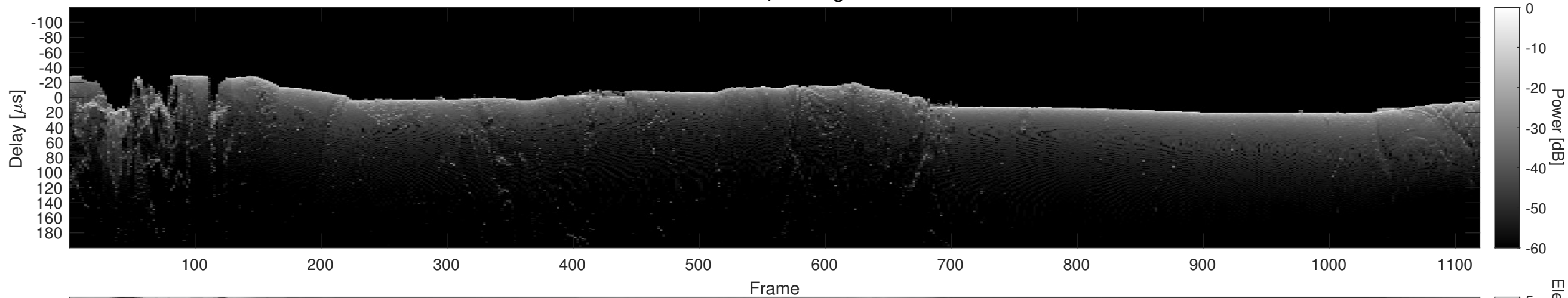
Orbit 12177, Cluttergram
