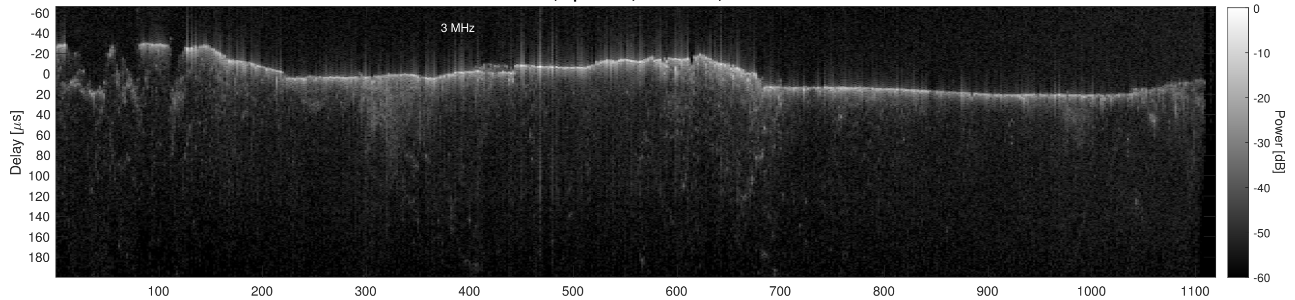
Orbit 12177, Cluttergram
