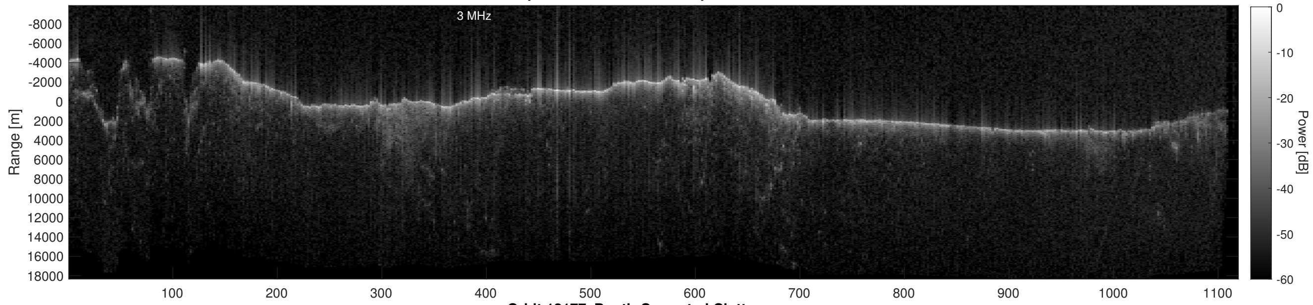
Orbit 12177, Depth-Corrected Cluttergram
