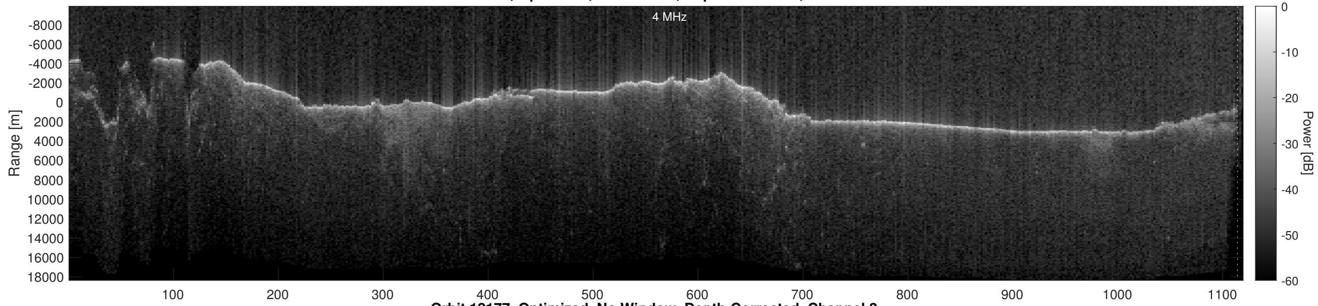
Orbit 12177, Optimized, No Window, Depth-Corrected, Channel 2
