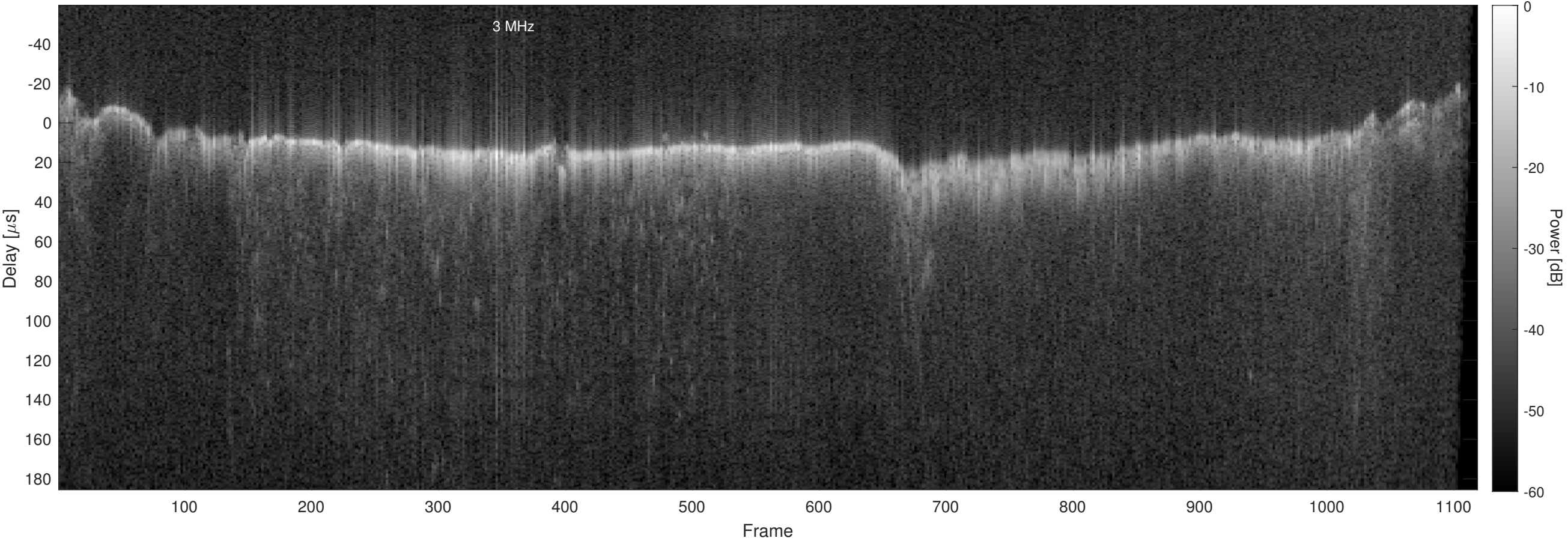
Orbit 12178, Chapman, No Window, Channel 2
