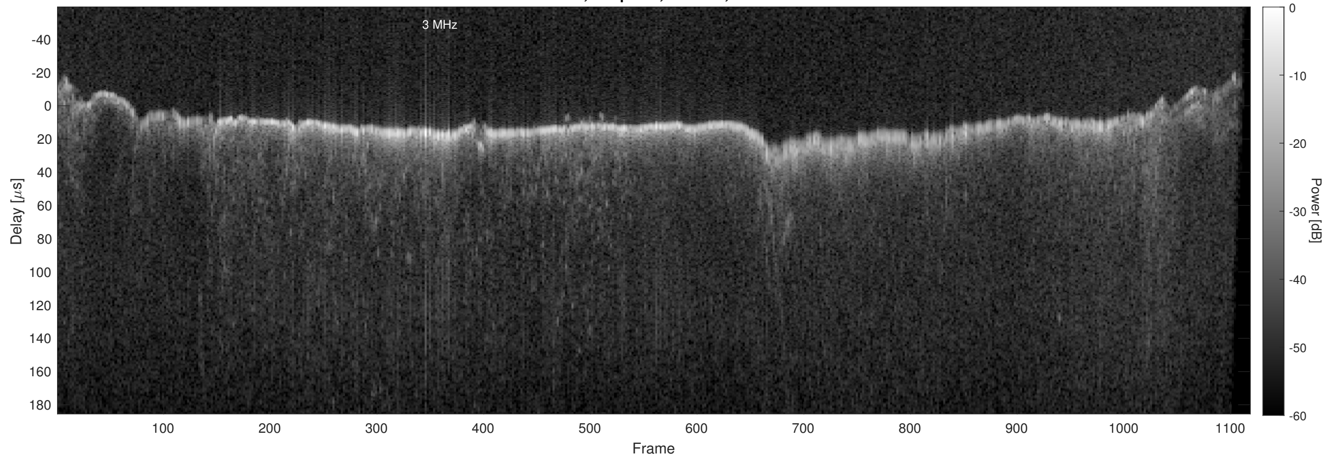
Orbit 12178, Chapman, Window, Channel 2
