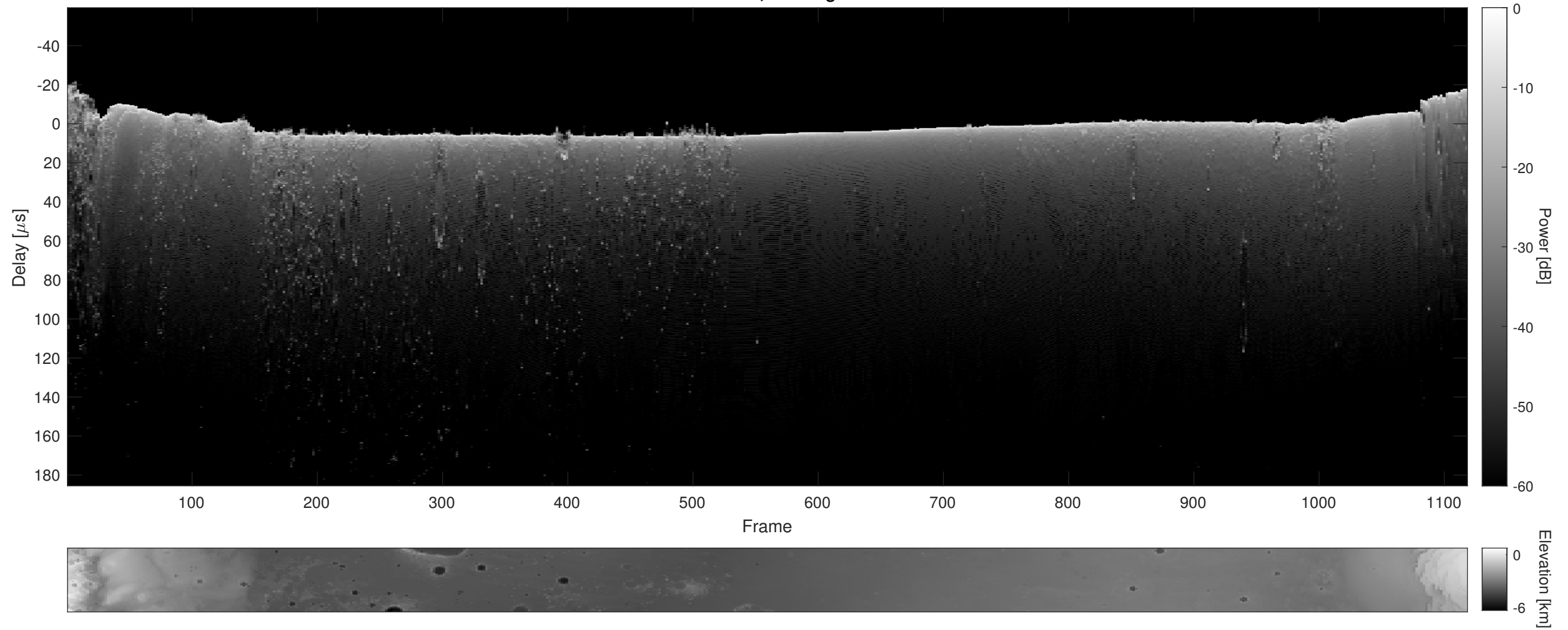
Orbit 12178, Cluttergram
