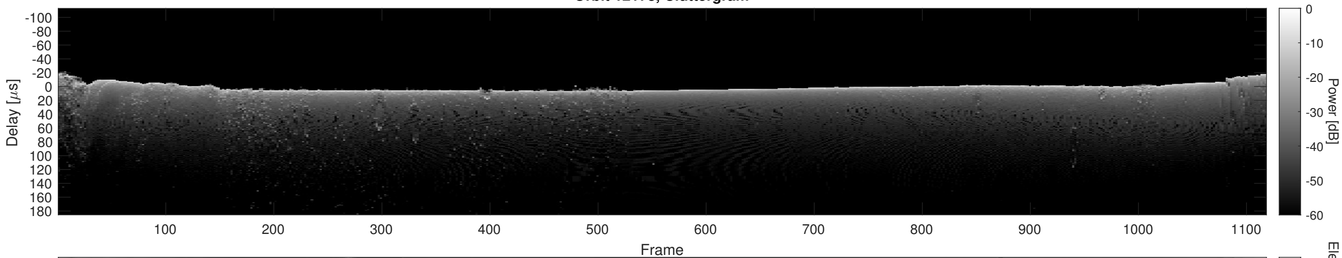
Orbit 12178, Cluttergram
