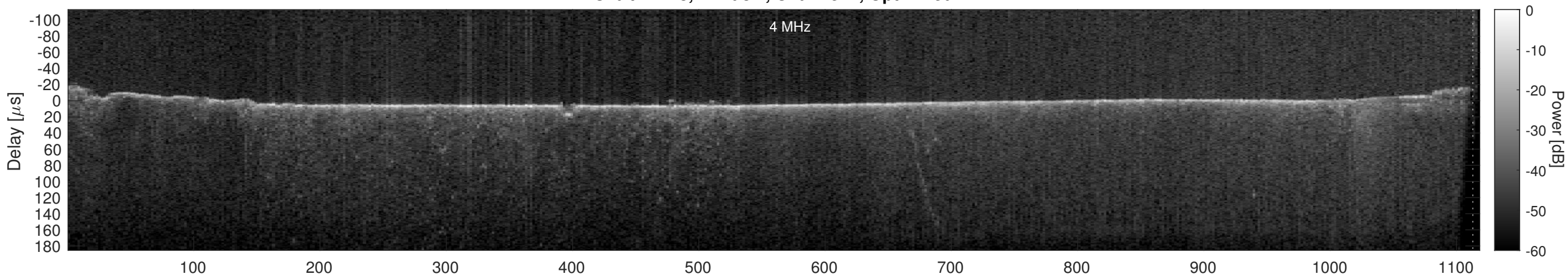
Orbit 12178, Cluttergram
