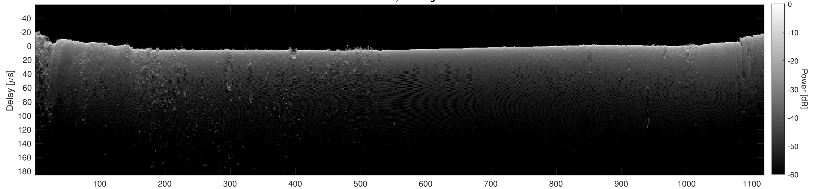
Orbit 12178, Cluttergram
