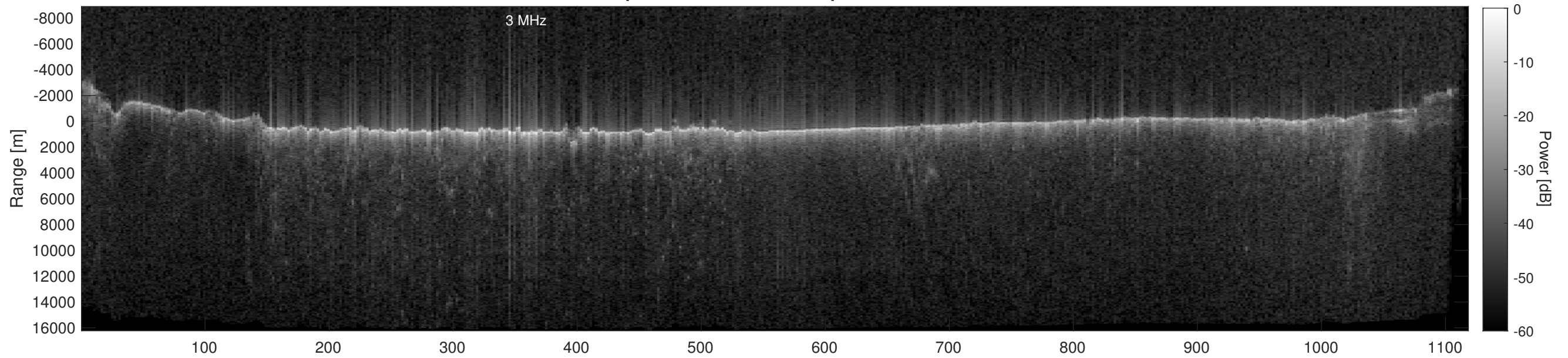
Orbit 12178, Depth-Corrected Cluttergram
