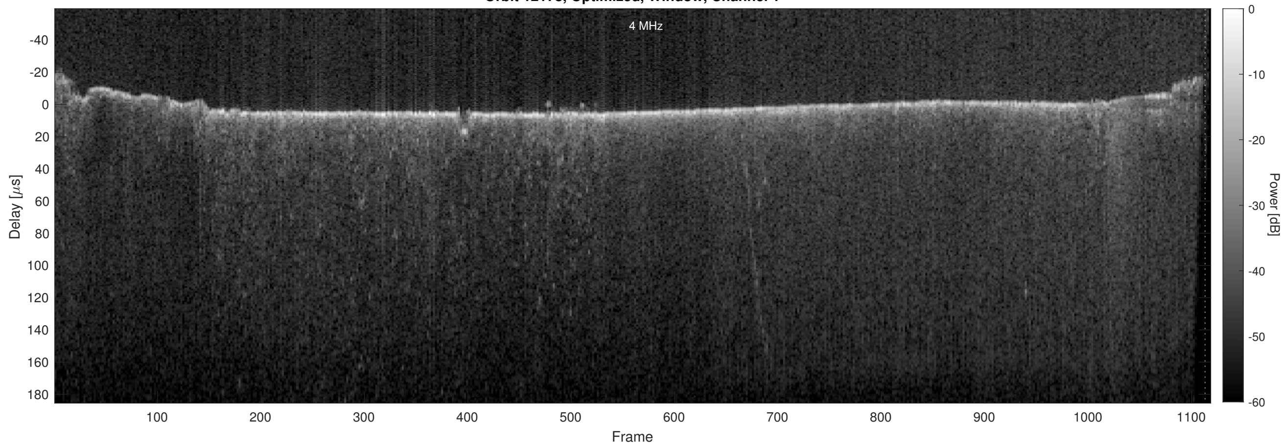
Orbit 12178, Optimized, Window, Channel 2
