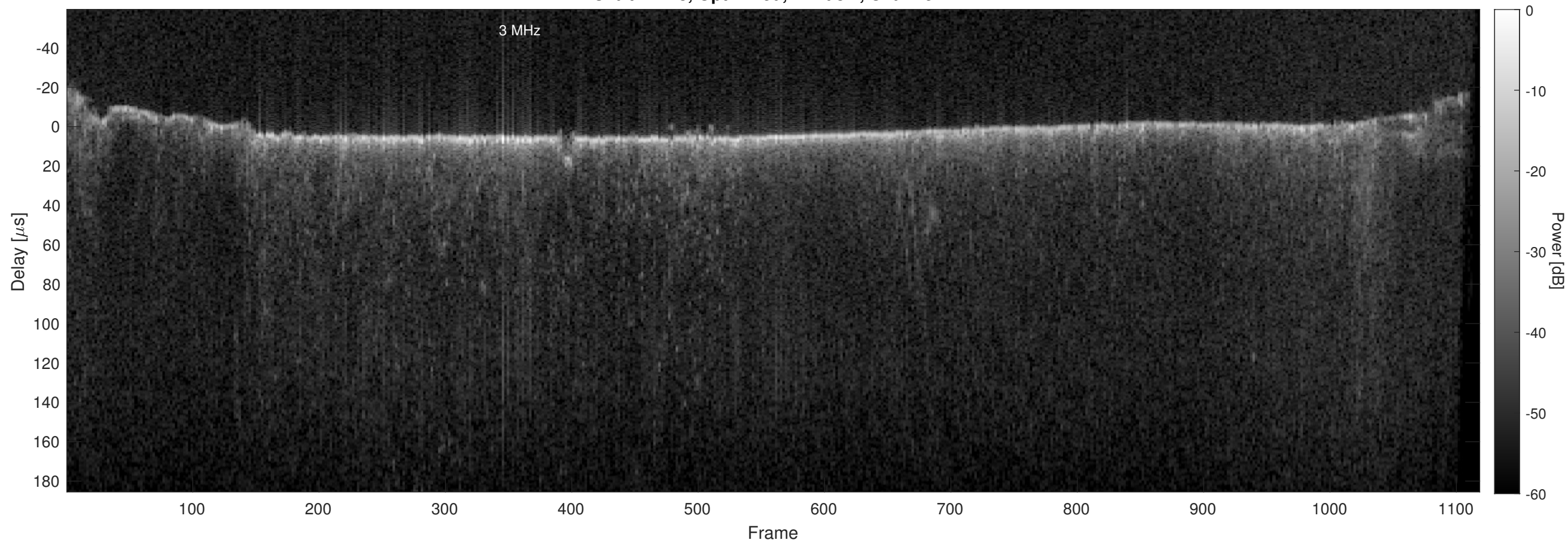
Orbit 12178, Optimized, Window, Channel 2
