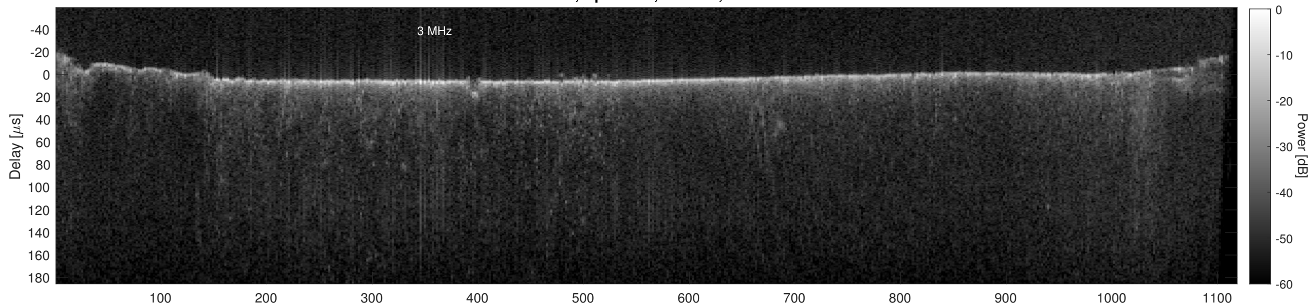
Orbit 12178, Cluttergram
