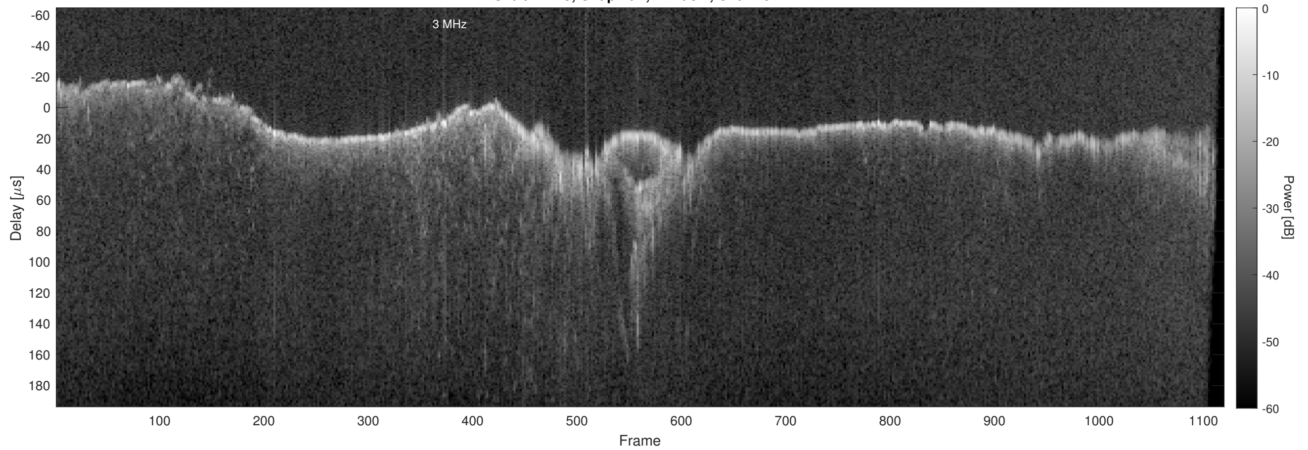
Orbit 12179, Chapman, Window, Channel 2
