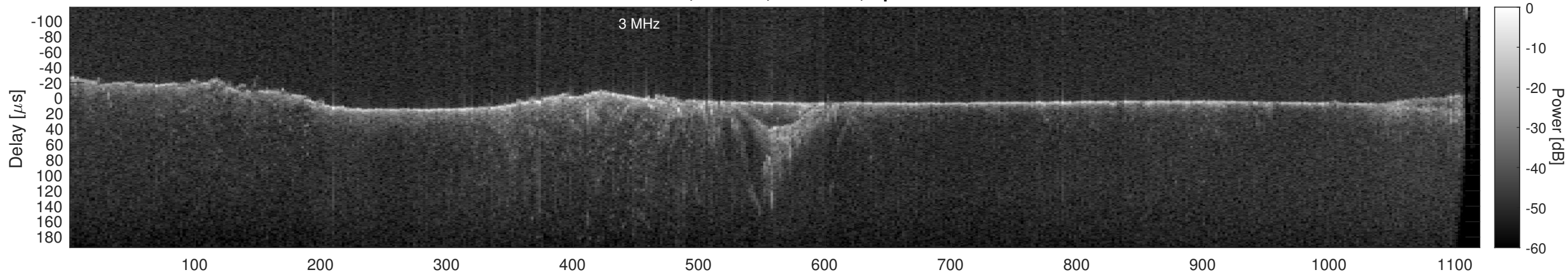
Orbit 12179, Cluttergram
