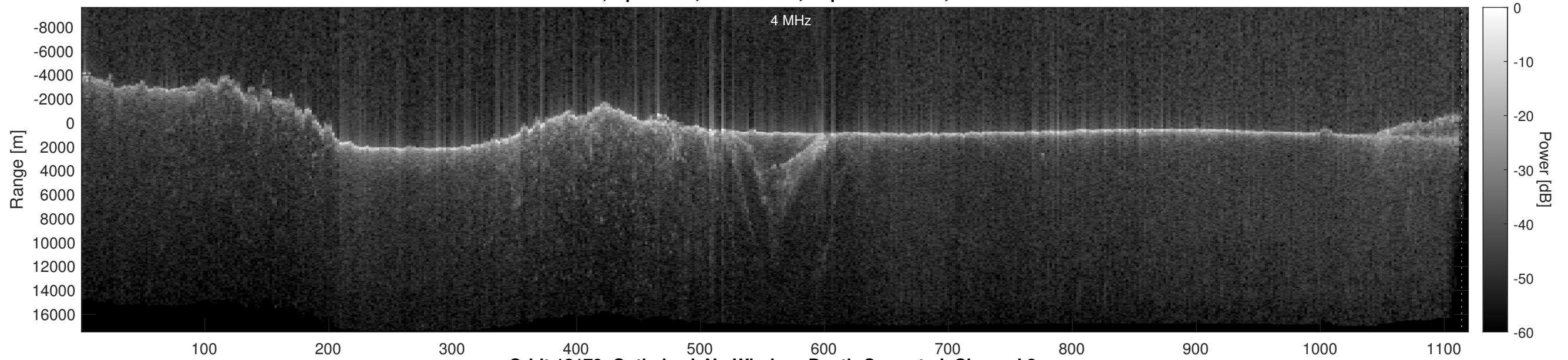
Orbit 12179, Optimized, No Window, Depth-Corrected, Channel 2
