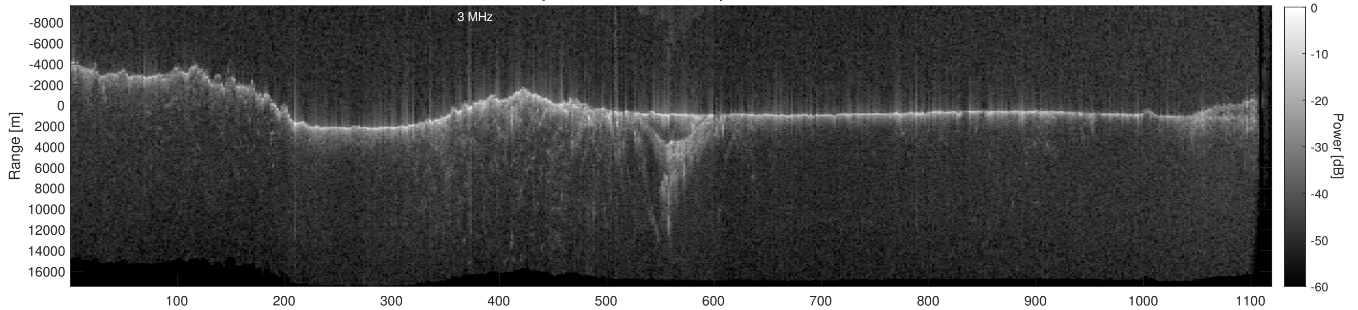
Orbit 12179, Depth-Corrected Cluttergram
