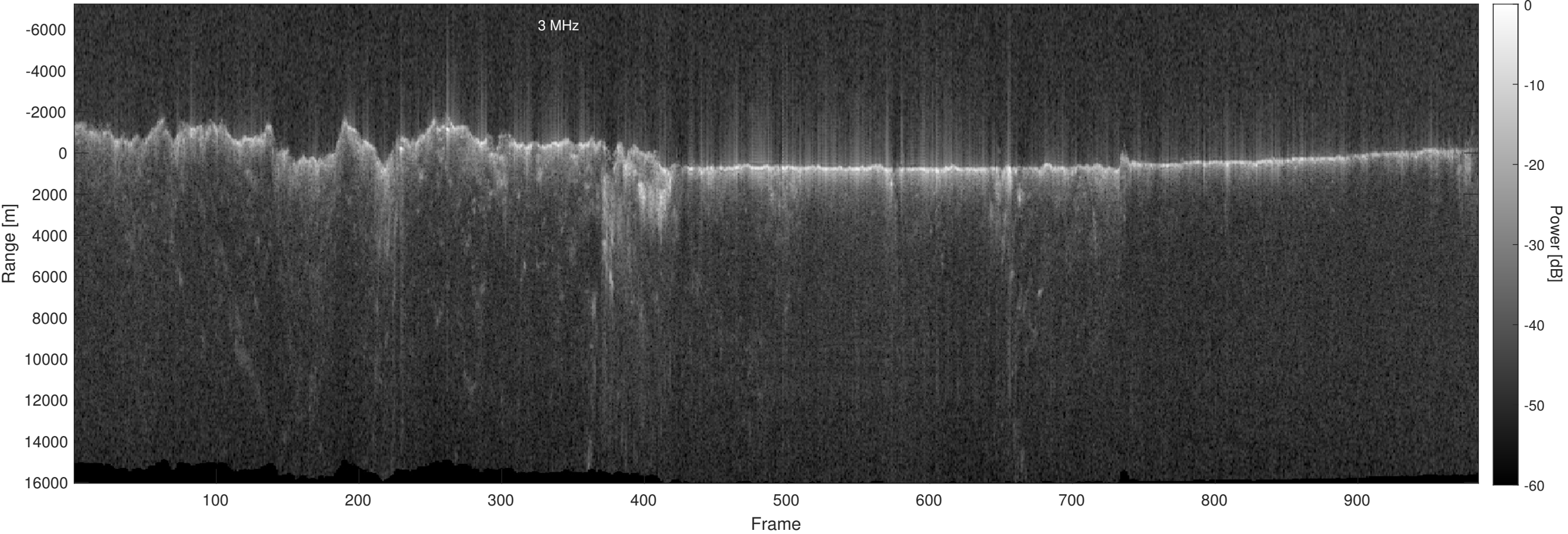
Orbit 12180, Optimized, No Window, Depth-Corrected, Channel 2
