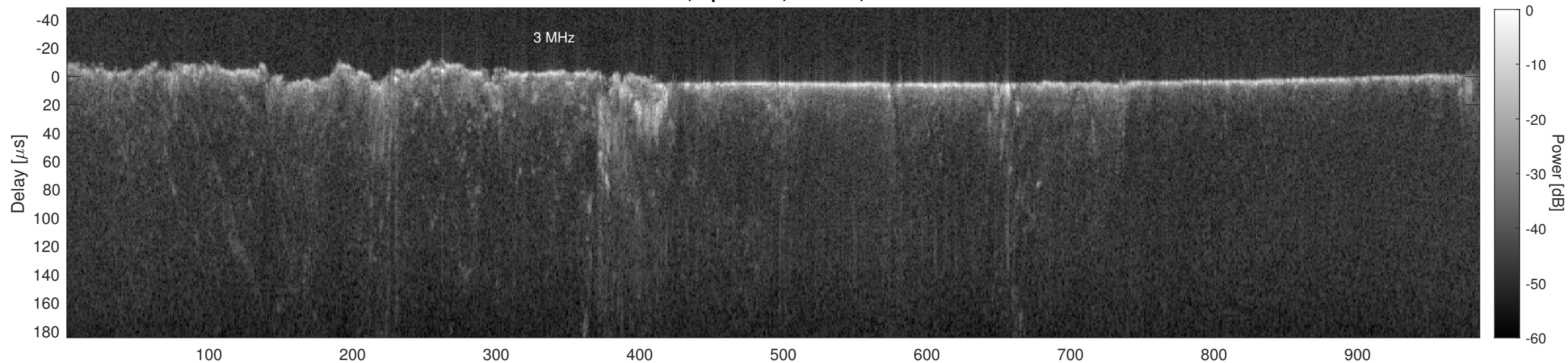
Orbit 12180, Cluttergram
