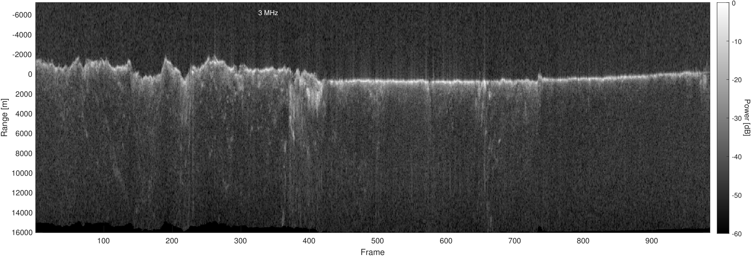
Orbit 12180, Optimized, Window, Depth-Corrected, Channel 2
