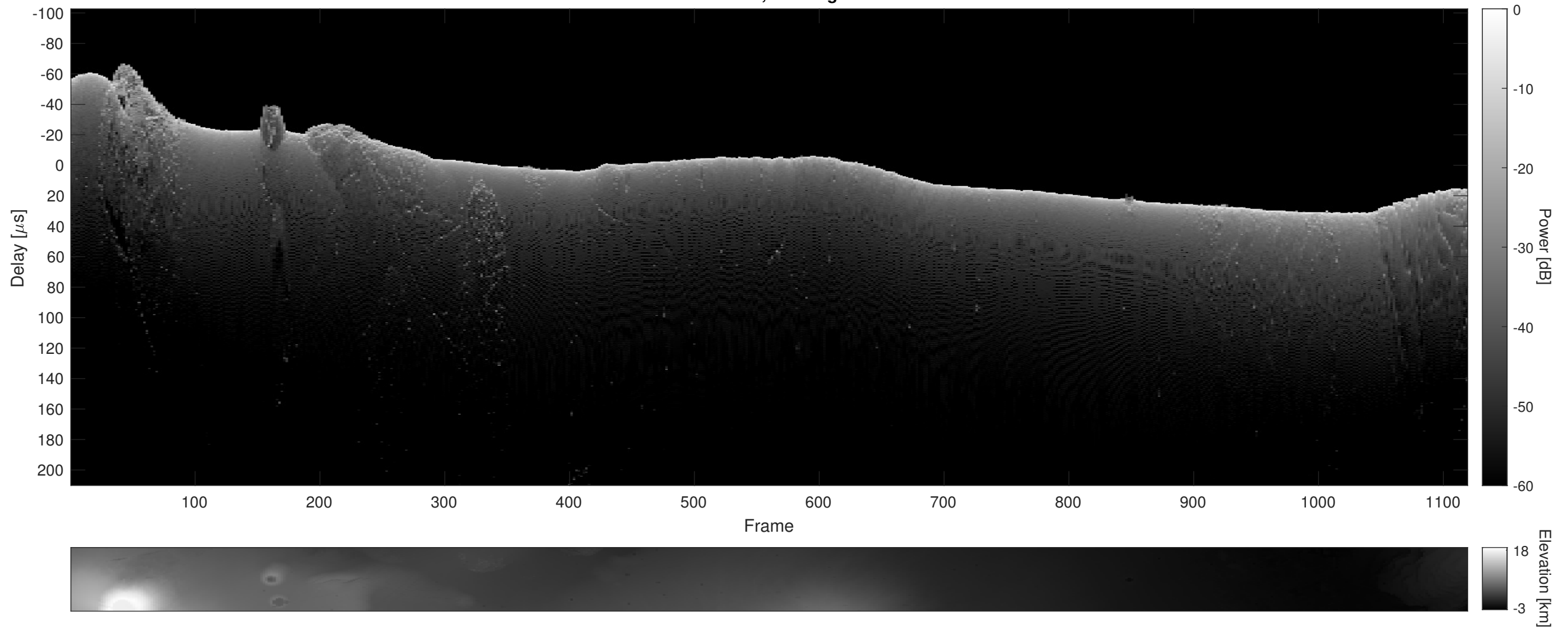
Orbit 12181, Cluttergram
