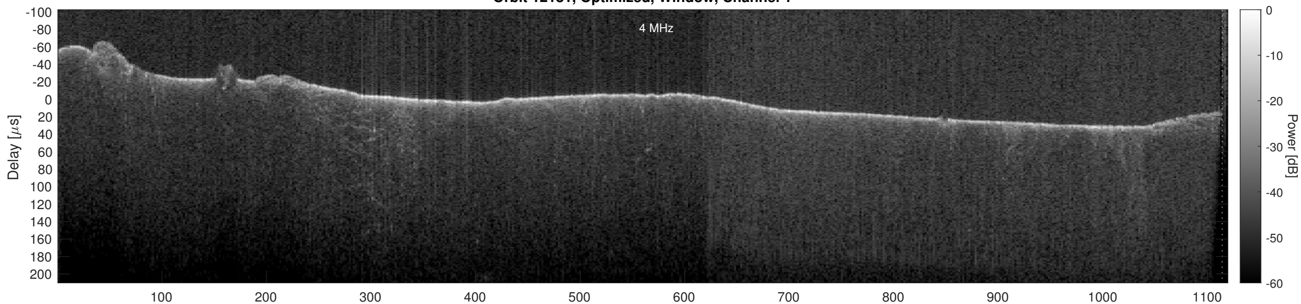
Orbit 12181, Optimized, Window, Channel 2
