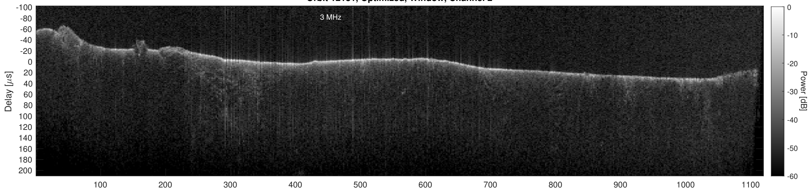
Orbit 12181, Cluttergram
